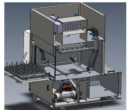
Series 136 Cabinet Style Bottle Washer
